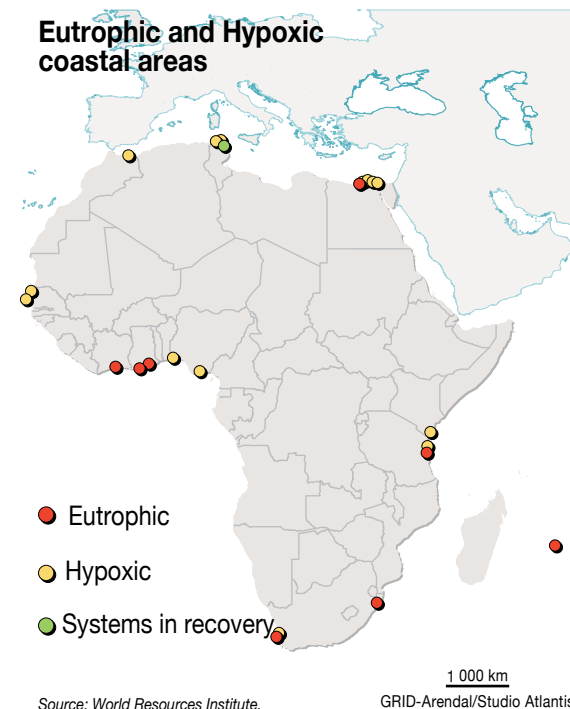
Figure 3.10. Eutrophic and hypoxic coastal areas of Africa
